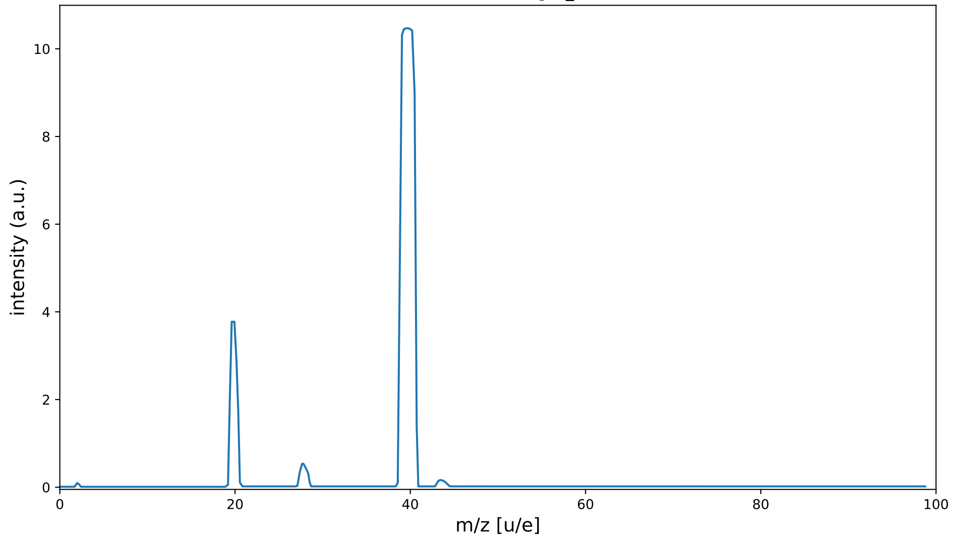
QMS-TPD: residual gas_4.txt
